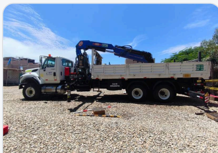
International PM 36026
